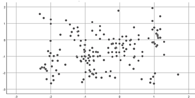
Gambar 2. Scatterplot Dependent Variable
