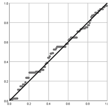
Gambar 1. Normal Probability Plot
